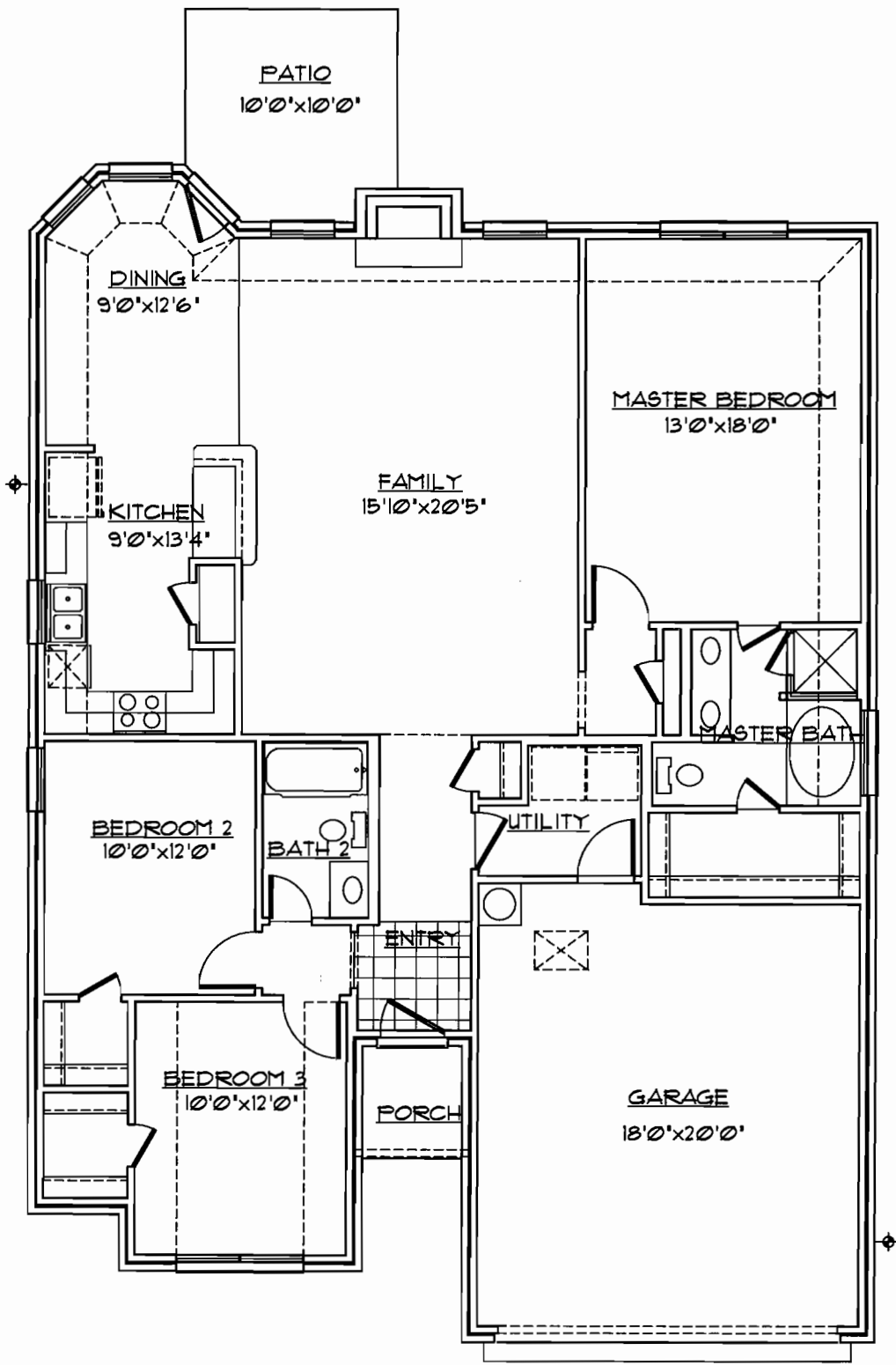
FLOOR PLAN 1/8"=1'0"
